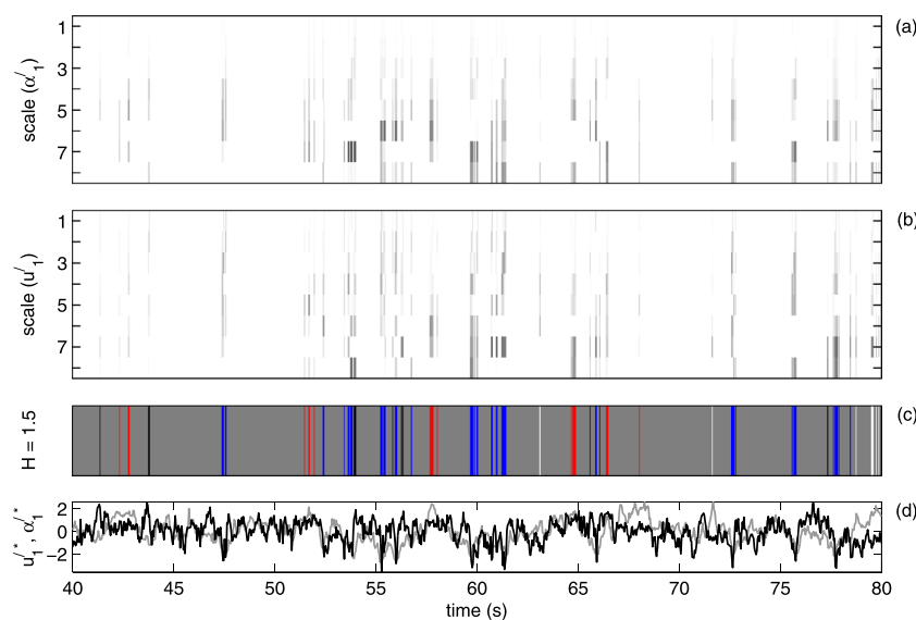
Figure 8. A wavelet and new quadrant decomposition of the velocity and Hölder exponent data at ( x=0.69 m, z=0.09 m) with hole size H=1.5 . This location is position (c) in Figure 2. The bottom plot shows time series for u_1 (black) and \alpha_1 (grey) with their means subtracted and normalized by their standard deviations; hence u_1^* and \alpha_1^* . Panel (c) indicates the times when the H=1.5 criterion is exceeded by vertical lines: Q2 (white), Q4 (black), Q1 (red) and Q3 (blue). The thickness of each line indicates the length of time that the threshold is exceeded. The upper plots are wavelet decompositions of the flow field for u_1(t) and \alpha_1(t) . Wavelet coefficients for the flow when H < 1.5 or that are opposite in nature to the sense of the flow event are ignored. The other coefficients are shaded proportional to their magnitude, with the shading normalized by the maximum absolute values across all scales, but separately for the two variables.
