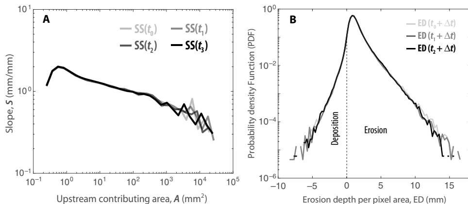
Fig. 2. Characterization of statistical SS landscapes. (A) Slope-area curves of the landscape at SS computed for four different instances, separated by 5-min intervals. Note that the curves show averages over logarithmic area bins. (B) PDFs of the pixel-wise ED computed by differencing the topographic data of the SS landscape at consecutive (5 min apart) instances. The shape of the PDF confirms the statistical nature of the SS landscape (a frozen landscape would have a Dirac delta PDF centered at the uplift depth corresponding to 5 min). The question we pose is whether every pixel of the SS landscape has an equal likelihood to experience any value of this PDF (an equal chance of experiencing above or below the landscape median erosion), as commonly assumed. We show that this is not the case, and there is a preferential scale-dependent organization of erosional fluxes, as shown in Fig. 3.
