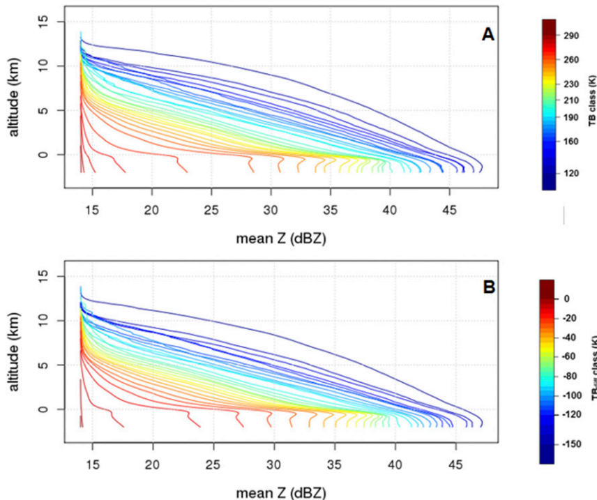
FIG. 4. (a) Mean along-beam KuPR reflectivity profile for various classes of 89V TB. (b) Mean along-beam KuPR reflectivity profile for various classes of TB_{diff} . Vertical axis is the altitude relative to the 0^{\circ}\text{C} isotherm. Adjacent classes with less than 400 observed profiles are merged for the computation of the average reflectivity profile. Color scale is chosen such that the classes corresponding to the same quantiles of the distributions of TB and TB_{diff} have the same color in (a) and (b).
