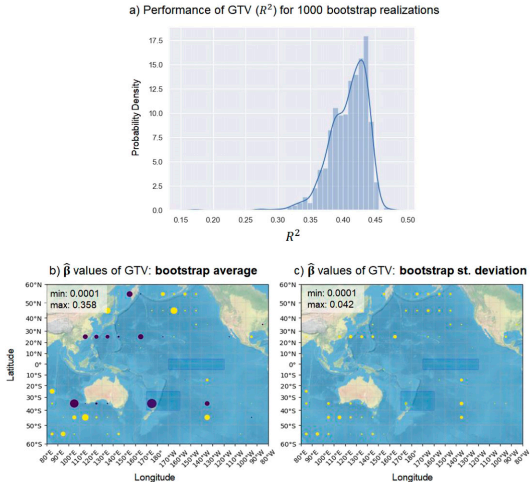
FIG. 8. Bootstrap investigation of the sensitivity of the GTV to the uncertainty of the covariance estimated from CESM-LENS. (a) The histogram of the coefficient of determination ( R^2 ) between the observed November–March SWUS precipitation and the GTV prediction across all 1000 bootstrap realizations. (b) The vector average of the 1000 \hat{\beta} vectors from the 1000 bootstrap realizations. For each realization, training is performed in the period from 1940/41 to 1989/90, using a fivefold cross-validation technique. (c) As in (b), but the standard deviation of the 1000 \hat{\beta} vectors is presented. The small uncertainty of the most important predictors (grids with the largest \hat{\beta} values) is noteworthy.
