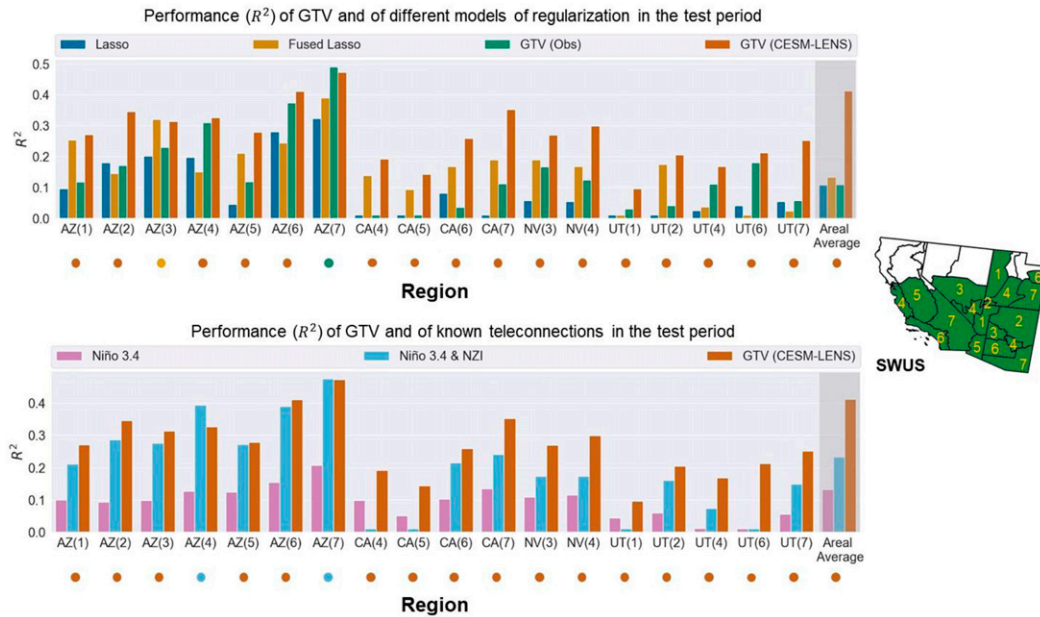
FIG. 6. Performance of (top) GTV and different methods of regularization and (bottom) known teleconnections in predicting precipitation totals over different SWUS divisions in the test period from 1990/91 to 2018/19. The coefficient of determination ( R^2 ) is presented. It is shown that GTV with model-estimated covariance of SSTs outperforms all other regularization methods (top) as well as statistical regression on two known teleconnections (bottom).
