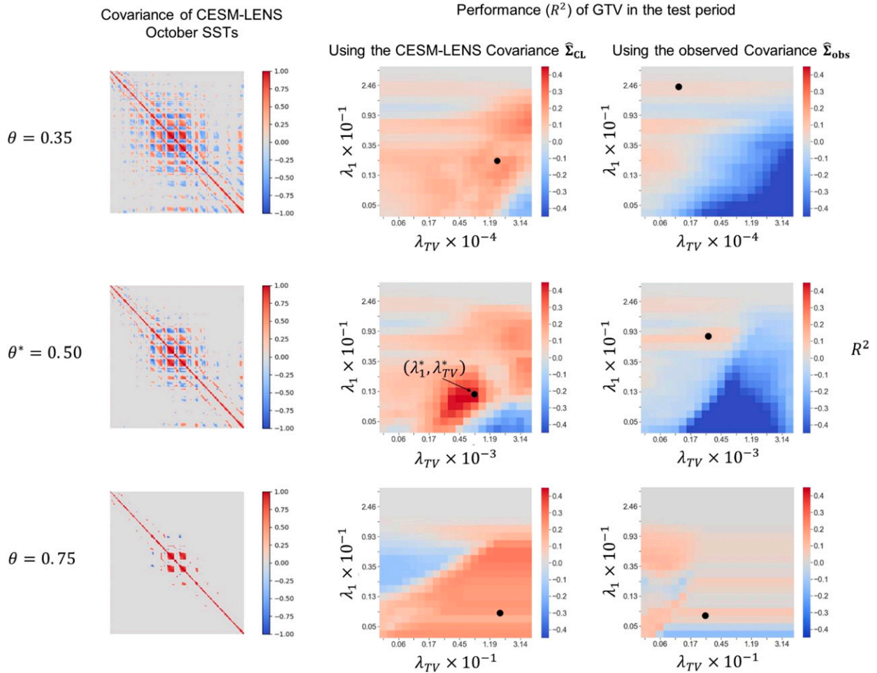
FIG. 4. Sensitivity analysis of the GTV model performance for a range of covariance thresholds \theta and regularization parameters \lambda_1 and \lambda_{TV} . (left) The covariance of the October SSTs (as estimated based on the CESM-LENS) for three different thresholds ( \theta = 0.35, 0.5 , and 0.75 ). (center) The coefficient of determination ( R^2 ) between the areal average observed and model predicted precipitation in the test period (1990/91–2018/19), when the CESM-LENS covariance is used to define the GTV regularizer. (right) As in the center panels, but when the observed SST covariance is used. In all panels, and conditional on the corresponding values of \theta , the optimal (\lambda_1^*, \lambda_{TV}^*) pair for each model (obtained by using a fivefold cross-validation in the training period 1940/41–1989/90) is shown (black dots). These results highlight that 1) the use of the CESM-LENS covariance, instead of the observational covariance, to inform the GTV regularizer leads to a highly robust and improved predictive performance, as judged by the larger domain of regularization parameters with high R^2 values (see center column plots, as compared to their right counterparts), and 2) our choice to use a threshold of \theta^* = 0.5 , which was based on a fivefold cross-validation in the training period (see section 4a), shows to yield the most robust and highest predictive performance.
