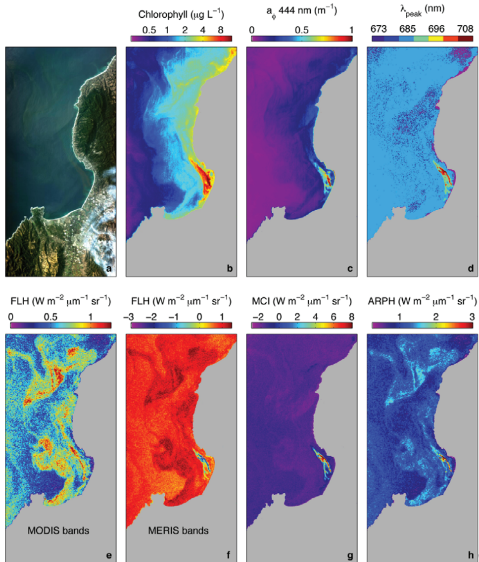
Figure 8.2. Phytoplankton characterization from a suite of algorithms using a HICO hyperspectral image acquired on 6 November 2012 over Monterey Bay, CA. The enhanced color image (a) used bands centered at the 466 nm (blue), 554 nm (green), and 708 nm (near infrared, to emphasize signal of a red tide). Hyperspectral data allow various band combinations to be used to optimize the imagery compared to multispectral sensors. SOURCE: Ryan et al., 2011.
